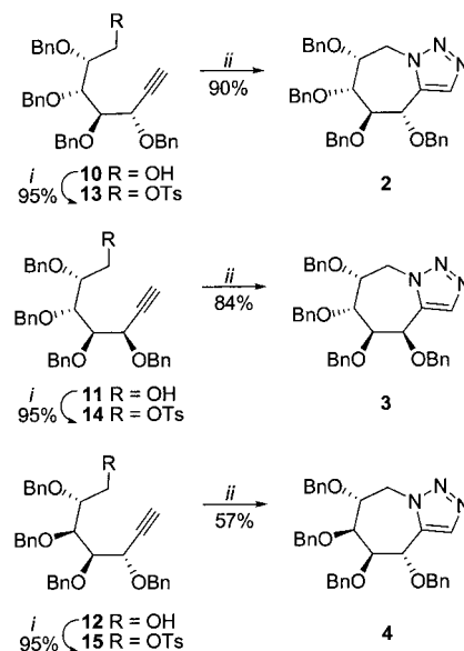
Scheme 4. Reagents and conditions: i ) TsCl, Py, room temp., 24 h. ii ) NaN 3 , DMF, 120 °C.
