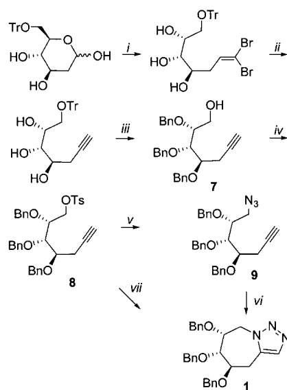
Scheme 3. Reagents and conditions: i ) \text{Ph}_3\text{PCHBr}_3 , Zn, 1,4-dioxane, reflux, 76%. ii ) n\text{BuLi} , THF, -70^\circ\text{C} , 92%. iii ) 1) \text{BnBr} , TBAI, NaH, DMF; 2) HCl concd., \text{CHCl}_3/\text{MeOH} , 76%. iv ) \text{TsCl} , Py, room temp, 95%. v ) \text{NaN}_3 , DMF, 80^\circ\text{C} , 5 min, 60%. vi ) Toluene, reflux, 24 h, 92%. vii ) \text{NaN}_3 , DMF, 120^\circ\text{C} , 3 h, 70%.
