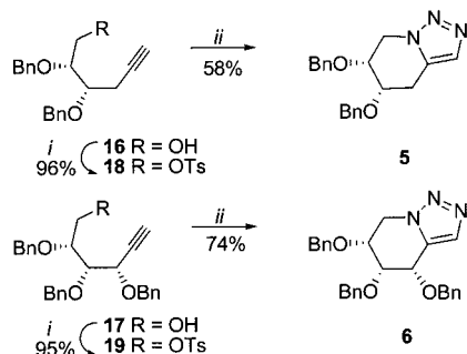
Scheme 5. Reagents and conditions: i ) TsCl, Py, room temp., 24 h. ii ) NaN 3 , DMF, 120 °C, 1 h.
